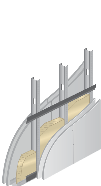
Partition Type 4 61 STC 3 5/8" Stud
