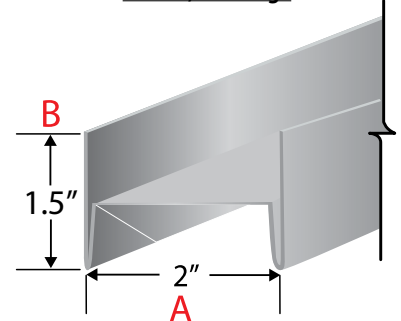
H-Stud, 25-Gauge
