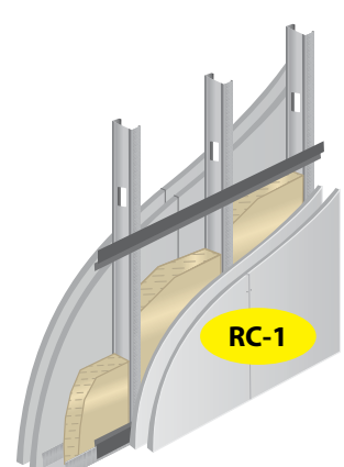
Partition Type 4 61 STC 3 5/8" Stud
