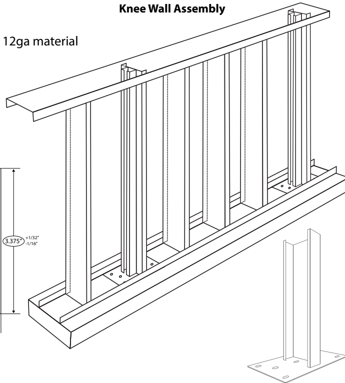
Knee Wall Assembly
