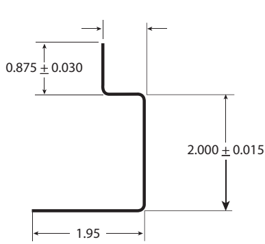
Non-Rated 195-NRVDT2
