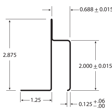
1 Hour Fire Rated 125-1HRVDT2
