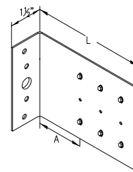
6 SCREW PATTERN
